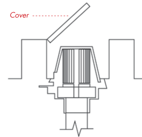
A typical inspection chamber at a roof drainage outlet in a vegetated roof area.
