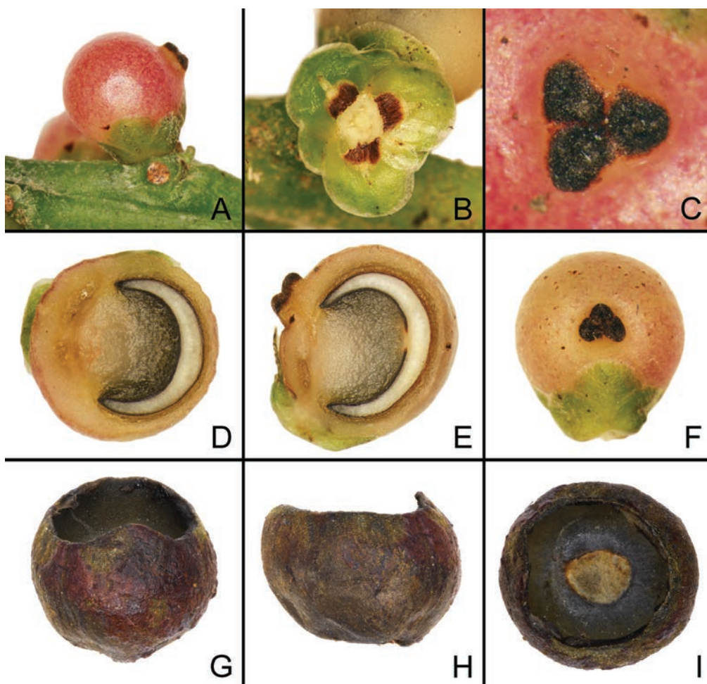
Fig. 2. Hanguana podzolicola Siti Nurfazilah et al. A. Side view detail of fruit attached to a branch showing tepals tightly clasping the base of the fruit. B. Detail of inner tepals, staminodes and staminodial scales. C. Detail of stigma. D. Cross section of fruit showing single seed and two empty locules. E. Longitudinal section of fruit. F. Fruit in top view, showing asymmetrically placed stigma. G. Seed (side view, appendage facing camera). H. Seed (side view, appendage to the right). I. Seed (top view, appendage to the left). From Leong-Škorničková, J. HAN-76 . (Photos: A–F: Jana Leong-Škorničková; G–I: Matti A. Niissalo)
